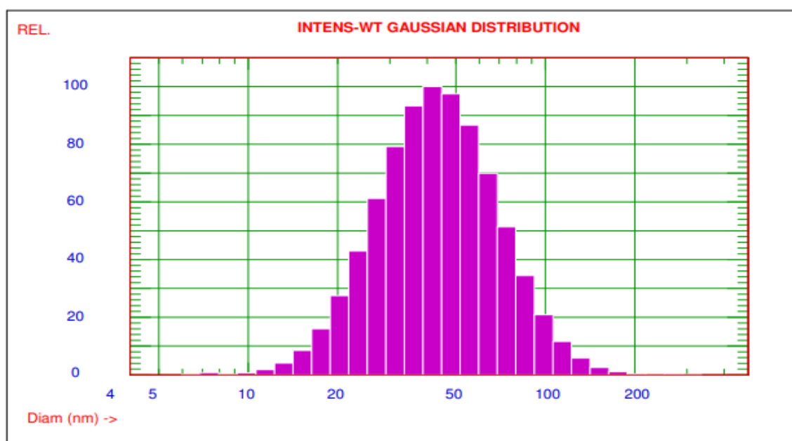
Plate 2. Characterization of synthesized MgO nanoparticles from neem leaf extract by particle size analyzer (Nicomp)
