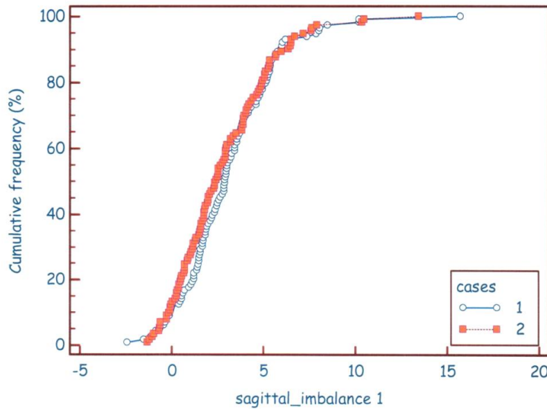
Fig. 1. Curves of cumulative frequency distribution in relation to the degree of sagittal imbalance (in degrees on the horizontal axis) before (cases 1; blue round dots and line), and after general osteopathic treatment (cases 2; red squares and line). The difference between the sagittal imbalance before and after GOT is statistically significant (two sided students t-test, p= 0.034)
