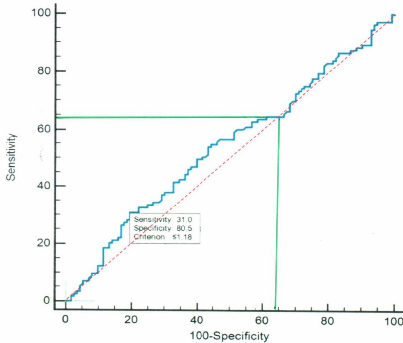
Fig. 2. Receiver operating characteristic (ROC) curve of sagittal imbalance, comparing the values before and after general osteopathic treatment. The red line depicts the diagonal. Points that are situated on the diagonal indicate that the measurements before and after general osteopathic treatment (GOT) were identical. In the cases belonging to the first and second tertile the ROC curve is situated toward the left cranial corner of the graph, indicating a reduction of the imbalance after GOT
