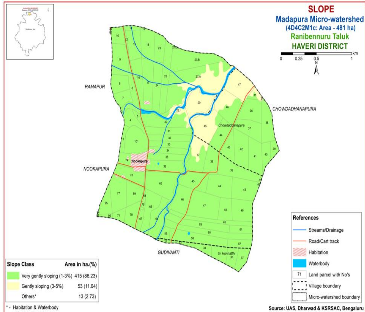
Fig. 7. Soil slope map of Madapura micro-watershed
