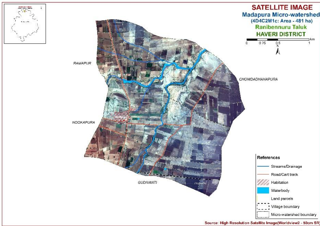
Fig. 2. Satellite image of Madapura micro-watershed
