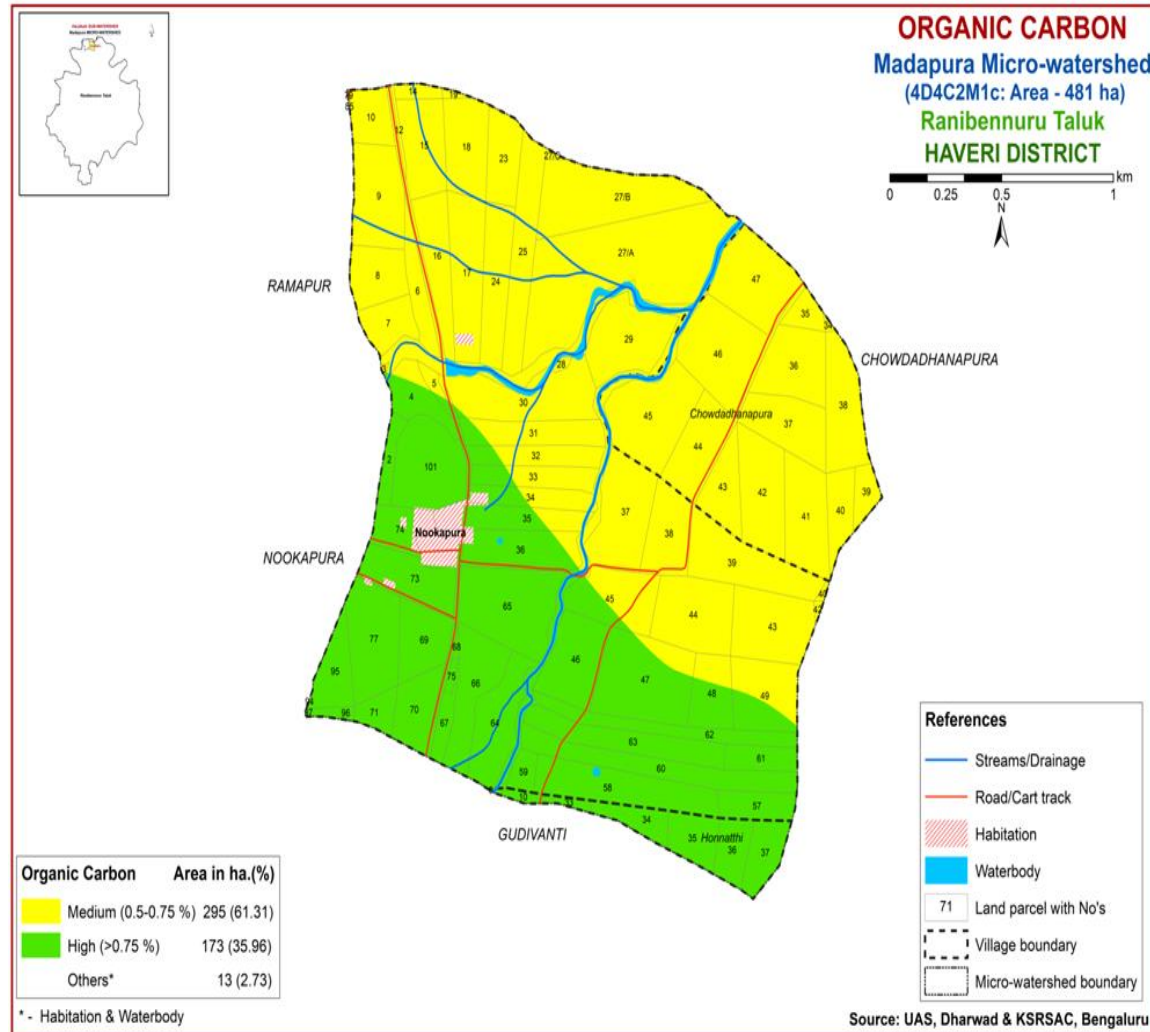
Fig. 11. Organic carbon map of Madapura micro-watershed
