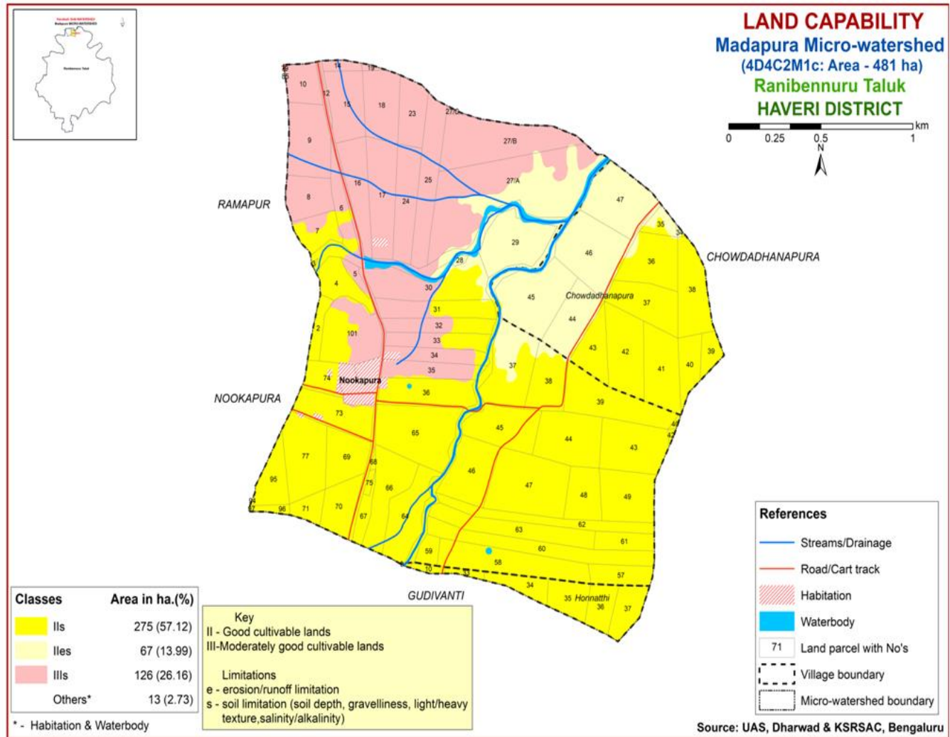
Fig. 20. Land capability classification in Madapura micr-waterhshed
