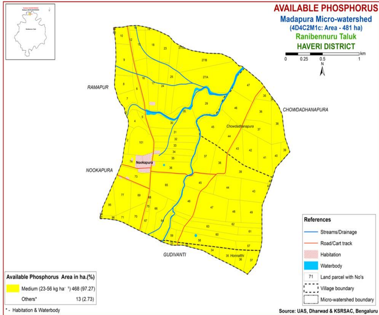
Fig. 13. Available phosphorous map of Madapura micro-watershed
