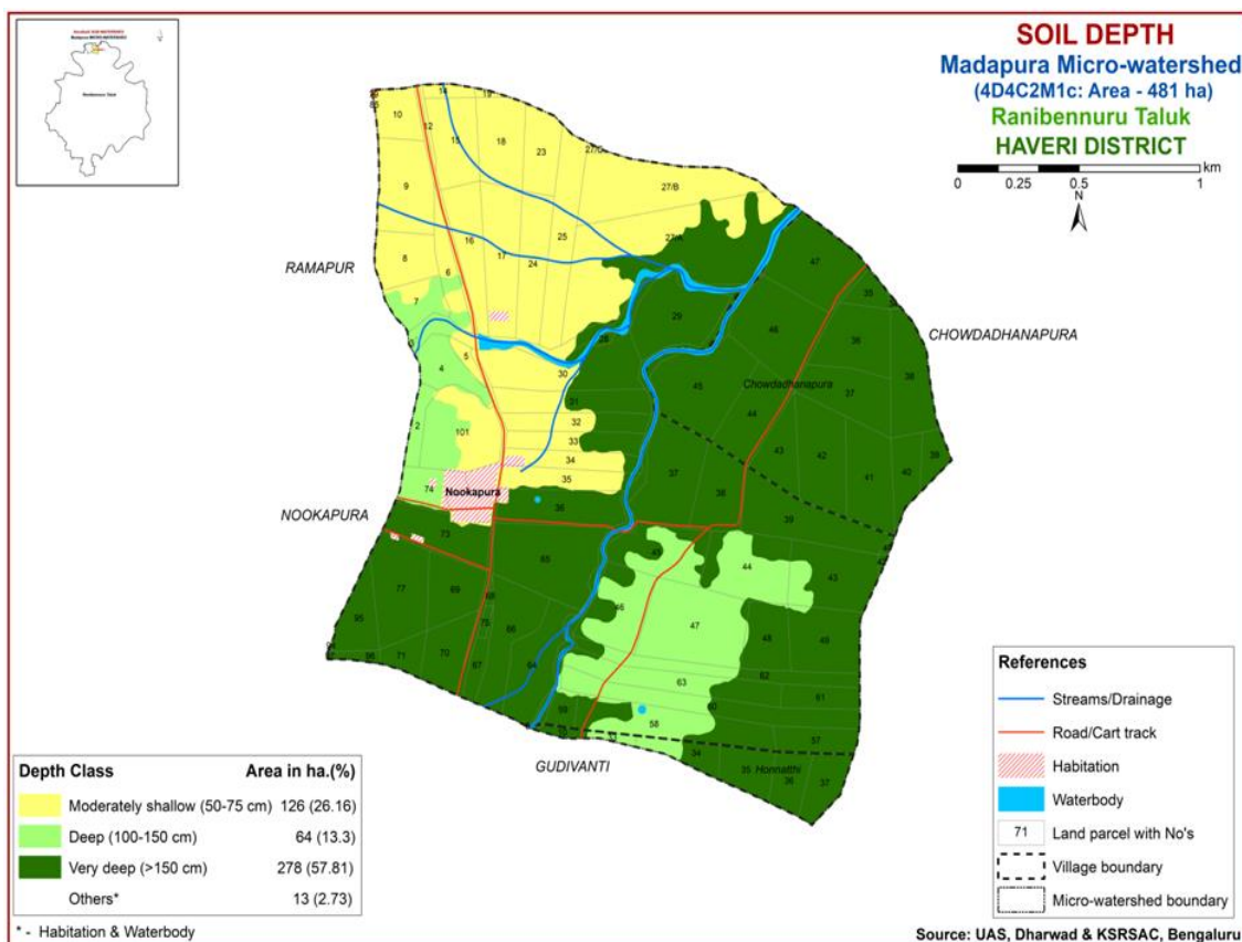
Fig. 4. Soil depth map of Madapura micro-watershed
