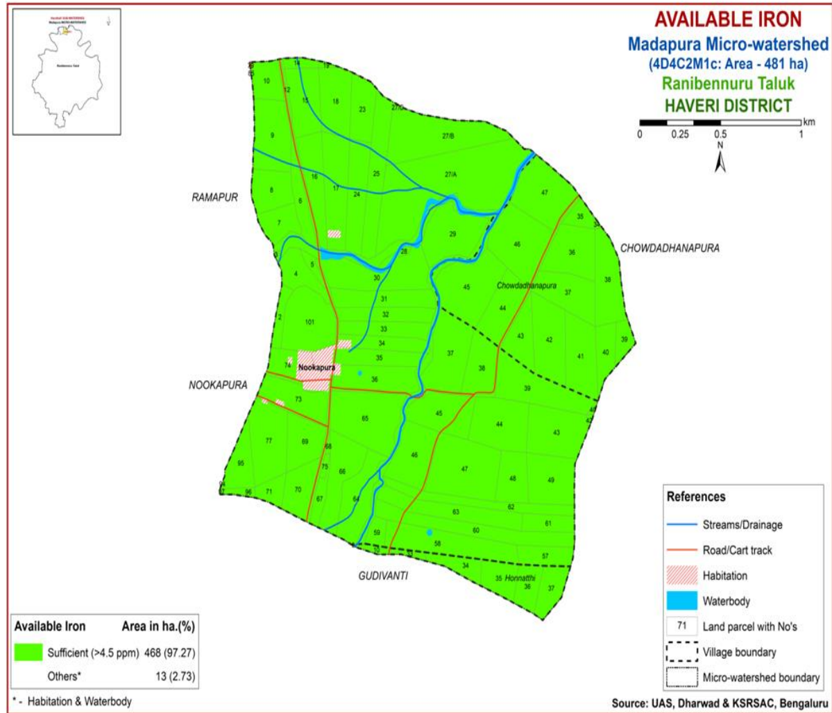
Fig. 16. Available iron map of Madapura micro-watershed
