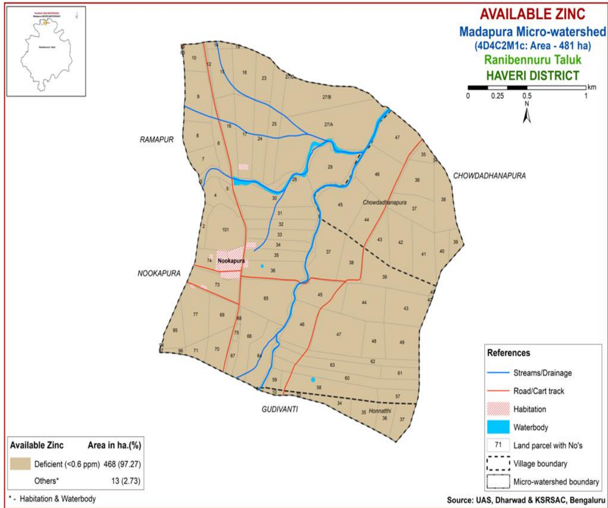
Fig. 19. Available zinc map of Madapura micro-watershed
