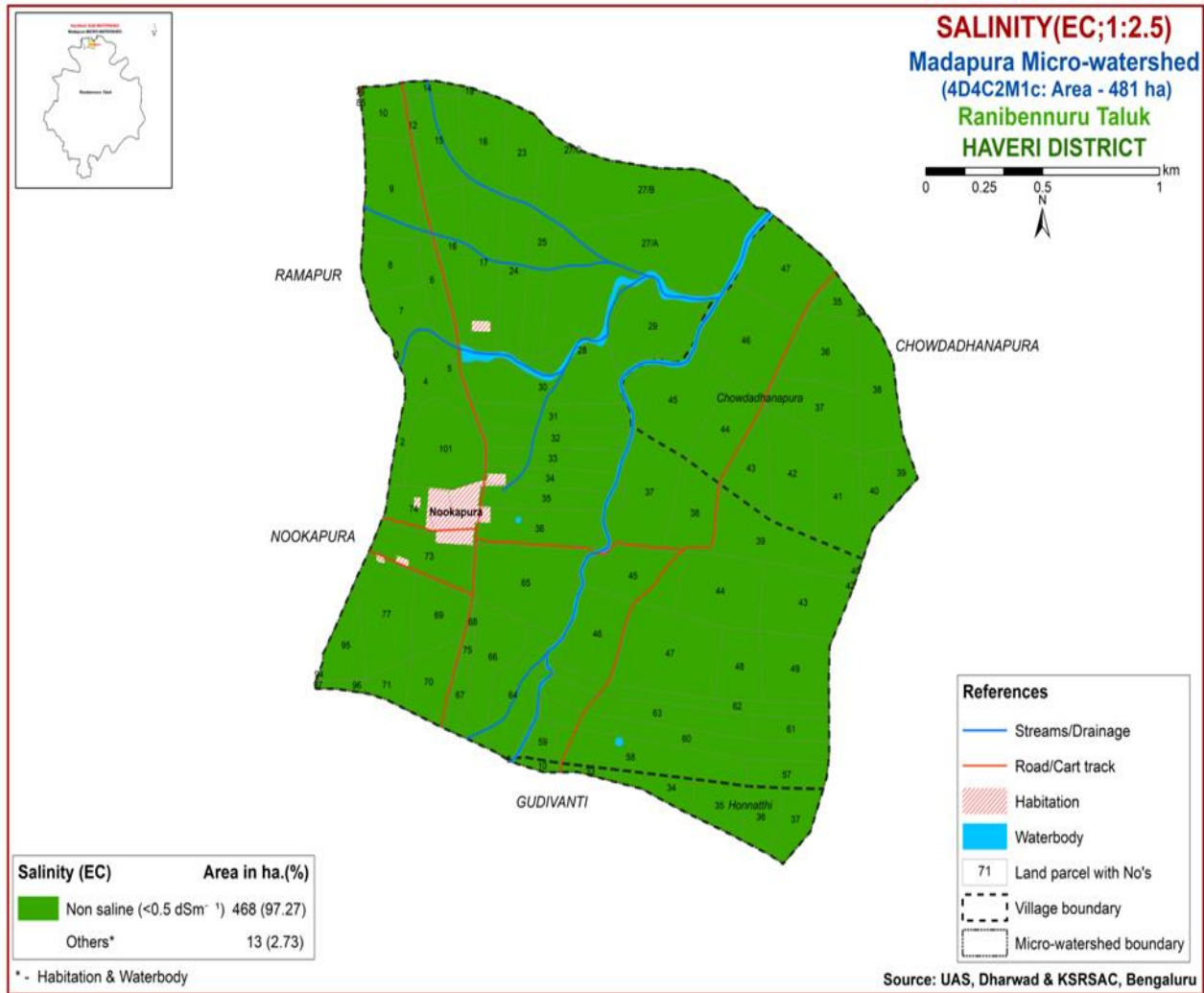
Fig. 10. Salinity map of Madapura micro-watershed
