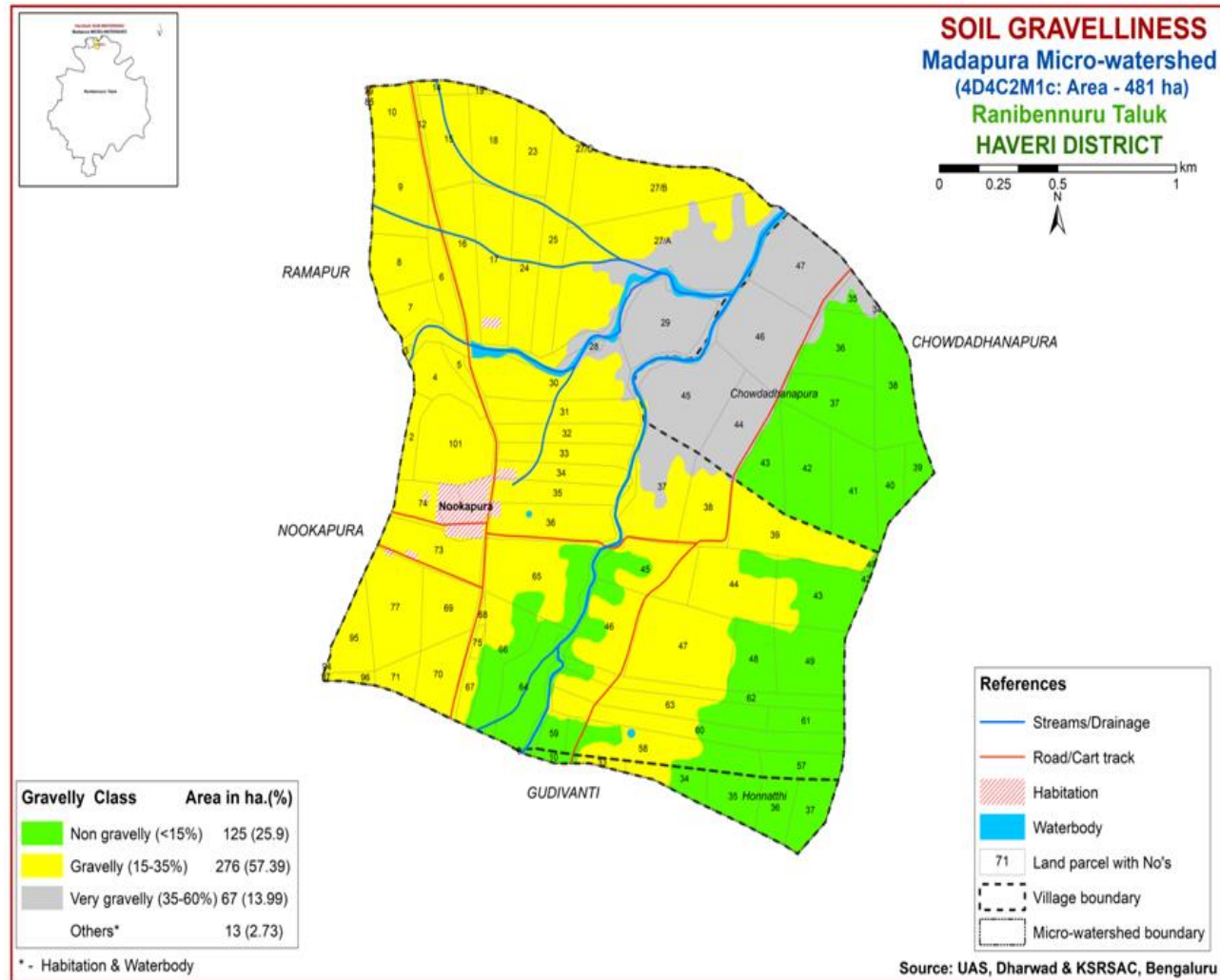
Fig. 6. Soil gravelliness map of Madapura micro-watershed
