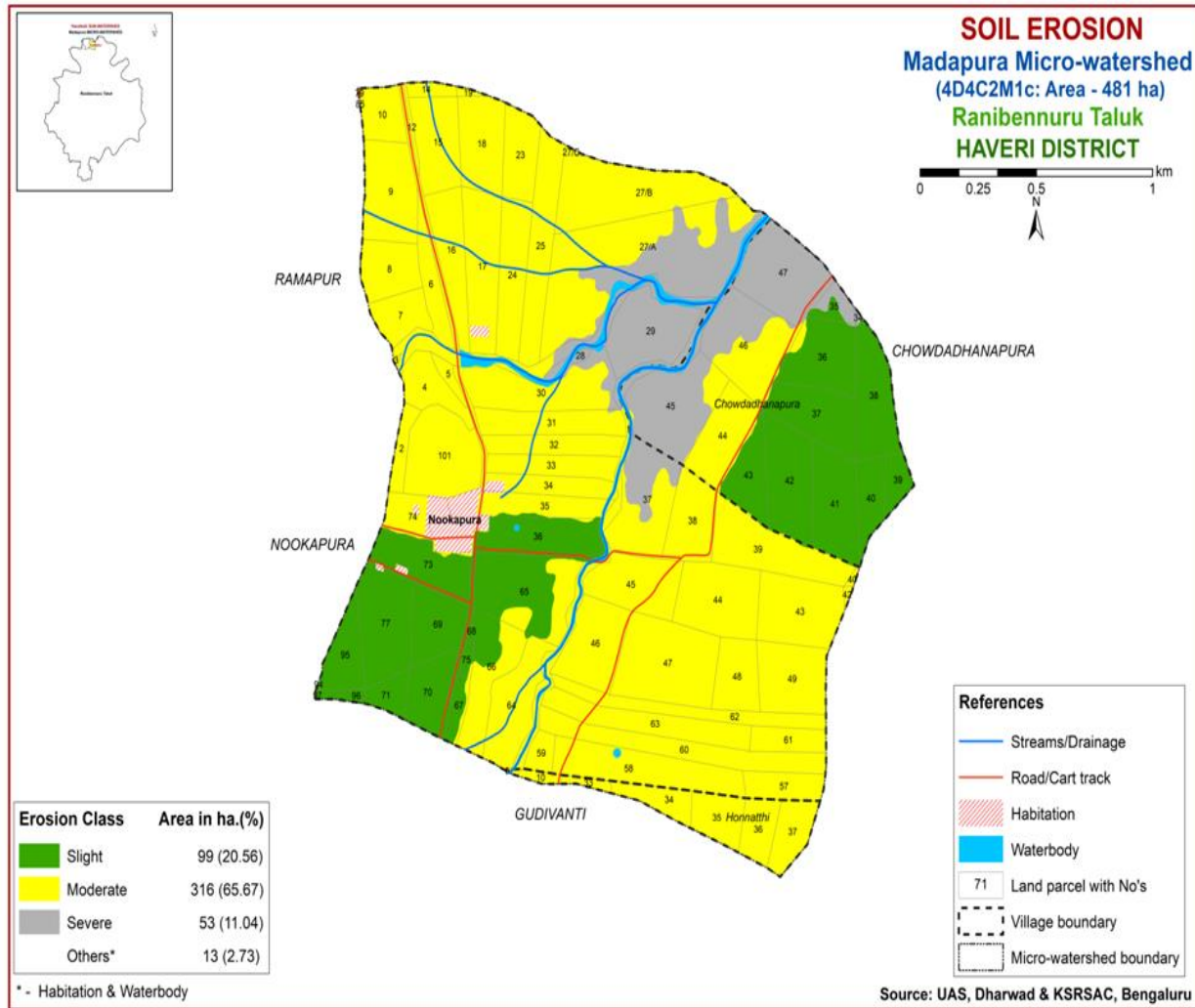
Fig. 8. Soil erosion map of Madapura micro-watershed
