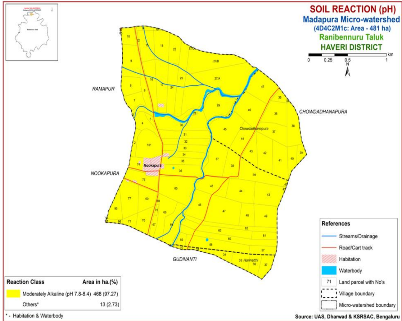
Fig. 9. Soil reaction map of Madapura micro-watershed
