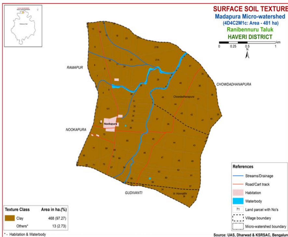
Fig. 5. Surface soil texture map of Madapura micro-watershed
