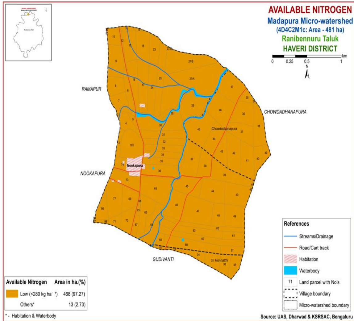
Fig. 12. Available nitrogen map of Madapura micro-watershed
