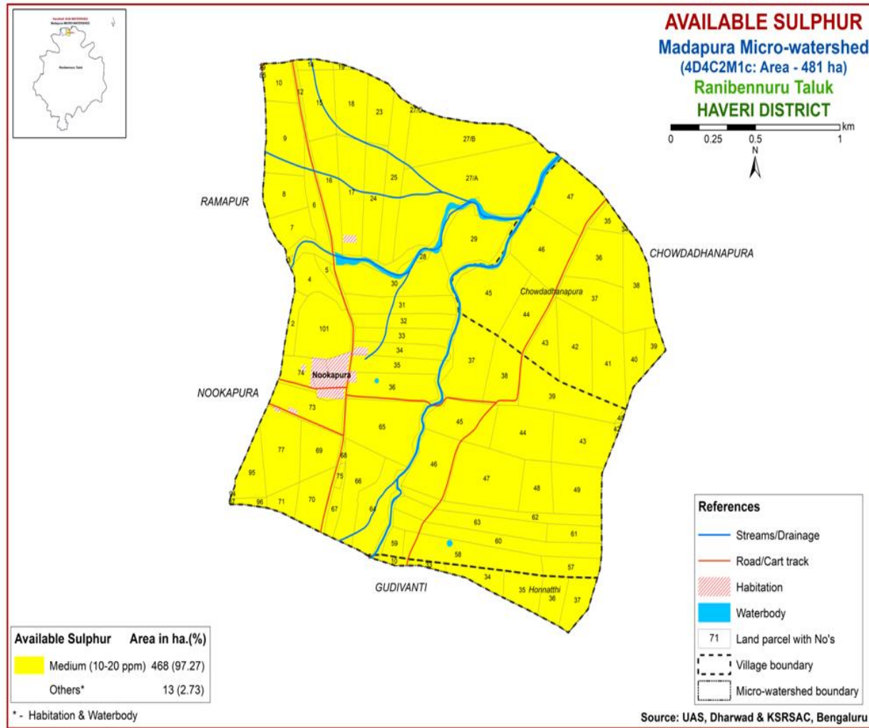
Fig. 15. Available sulphur map of Madapura micro-watershed
