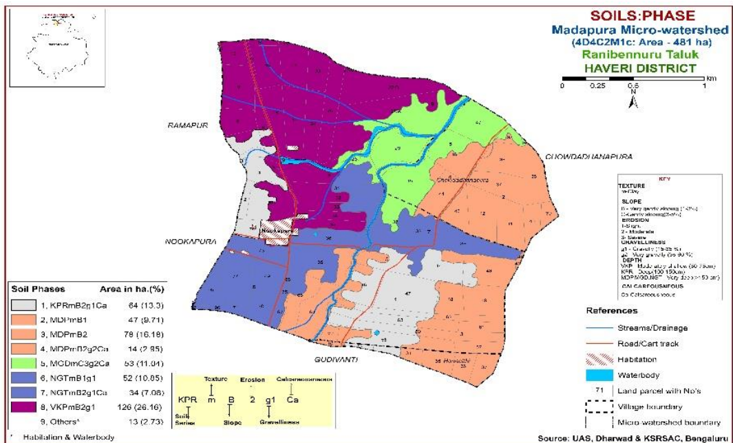
Fig. 3. Soil phase map of Madapura micro-watershed
