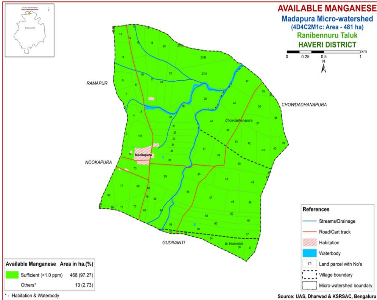
Fig. 18. Available manganese map of Madapura micro-watershed
