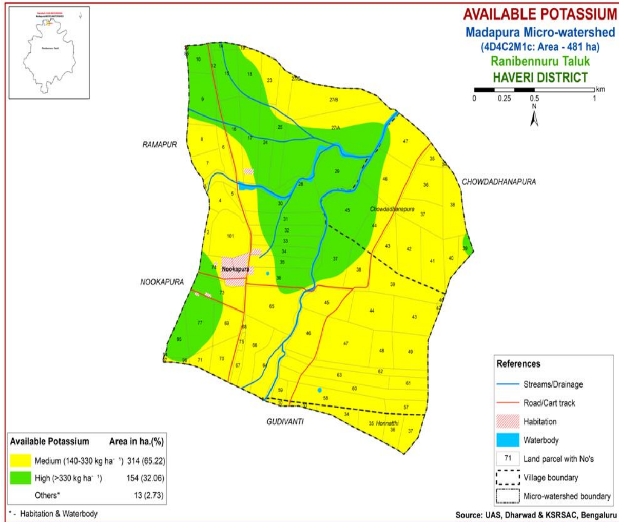
Fig. 14. Available potassium map of Madapura micro-watershed
