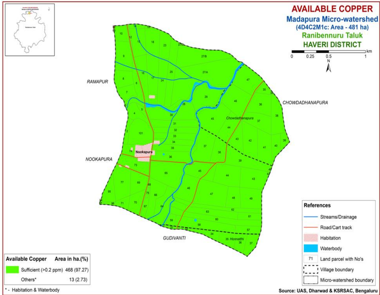
Fig. 17. Available copper map of Madapura micro-watershed
