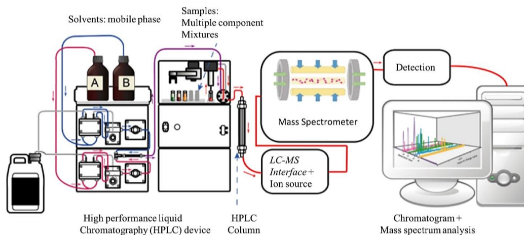
Fig. 2. Schematic representation of a Liquid Chromatography Mass Spectrometer. [Credit: Cwszot, Dagui1929, CasJu, and YassineMrabet, reproduced under the Creative Commons CC0 1.0 Universal Public Domain Dedication license.]
