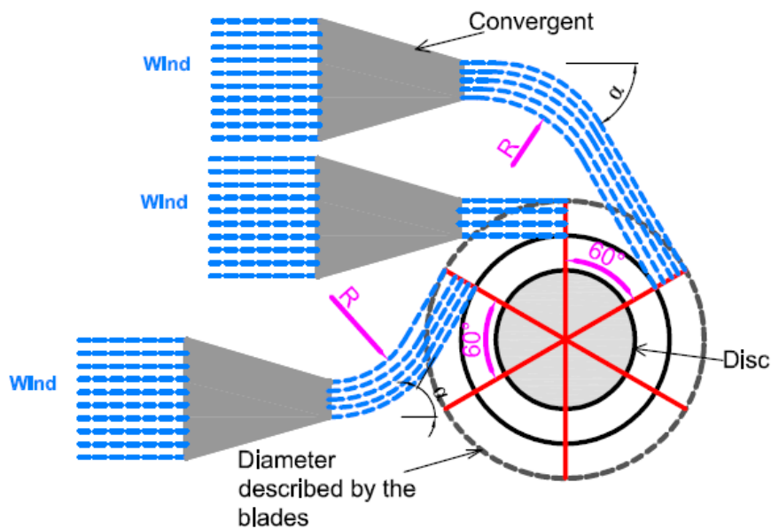
Fig. 2. Device with 3 convergents used in environment
