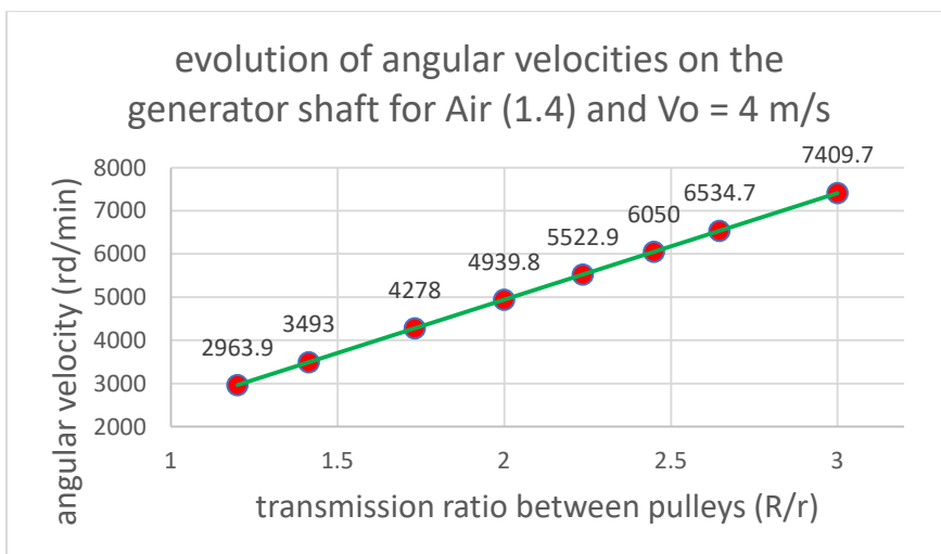
Fig. 6. Effect on the angular speed of the generator as a function of the pulley transmission ratio
