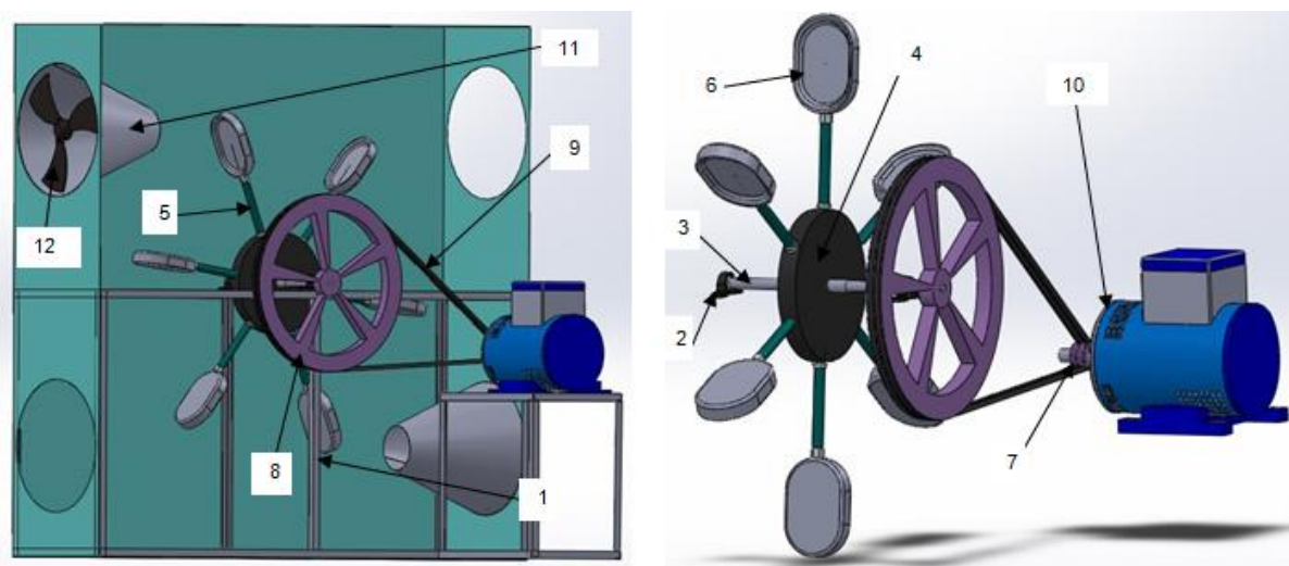
Fig. 1. Mechanical model of the convergent flow wind device
