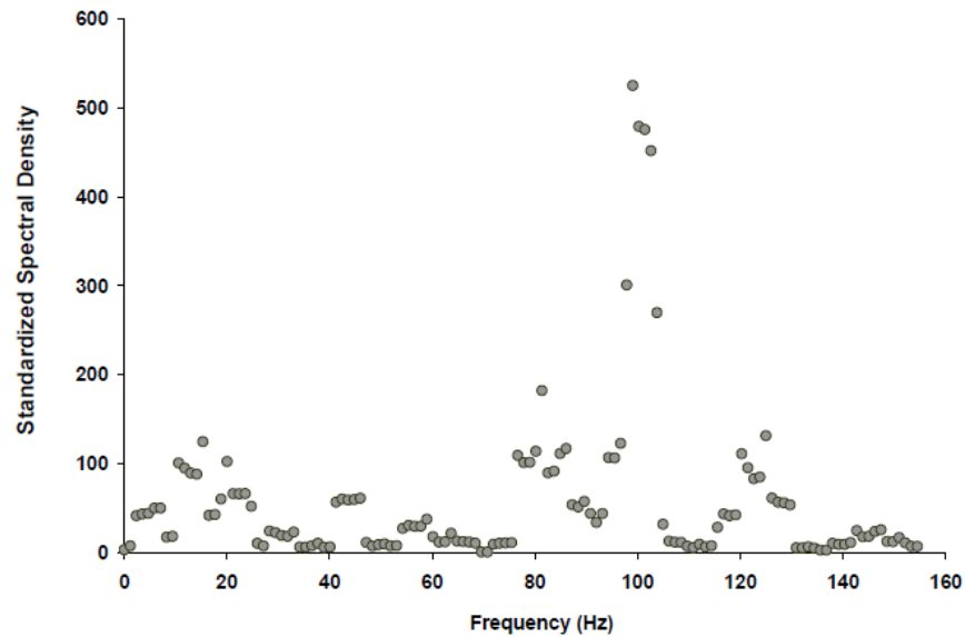
Fig. 3. Standardized spectral density of the accelerating phase modulated pattern generated within a decelerating angular velocity of the rotating magnetic fields within which the water samples were placed
