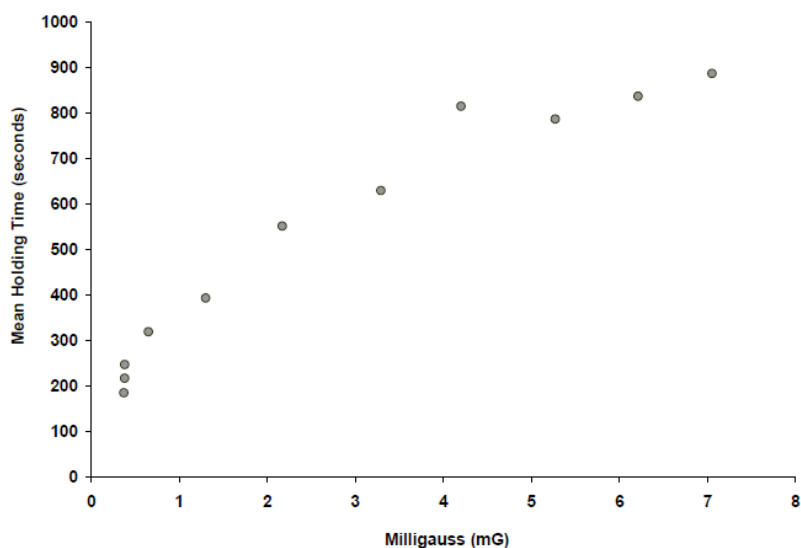
Fig. 4. Mean holding duration (in seconds), or the latency before the sudden decrease in pH in response to additions of a weak acid to the spring water as a function of the intensity of the rotating magnetic accelerating-decelerating angular velocity magnetic field
