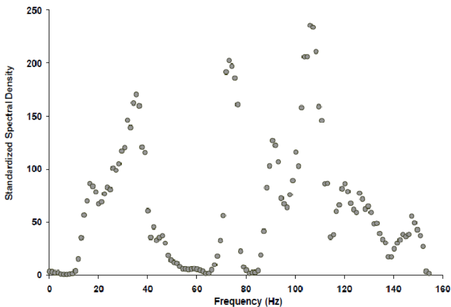
Fig. 2. Standardized spectral density of the decelerating phase modulated pattern generated with an accelerating angular velocity of the rotating magnetic field within which the water samples were placed
