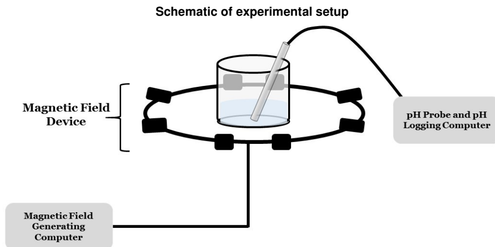
Fig. 1. Schematic of apparatus for generating changing angular accelerating magnetic fields around a volume of spring water within which pH was measured over time. The rates of change and patterns of the magnetic fields delivered through 8 solenoids were controlled by computer software and custom-constructed digital-to-analogue converters
