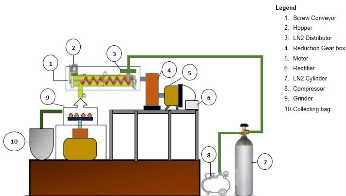
Fig. 1. Cryomilling system
