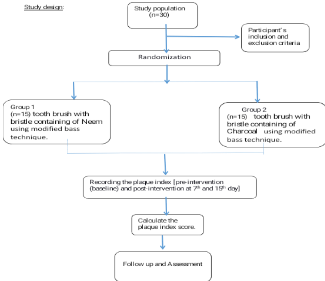
Fig. 1. Study design
